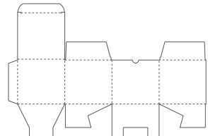
Fefco Code: 0215
